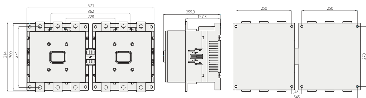
HGC800R
